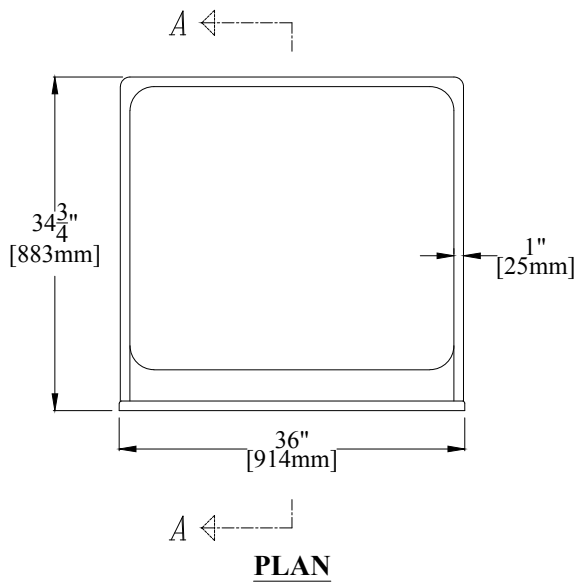
36" [914mm] Dome for Models 5636, 6636 & 9636
